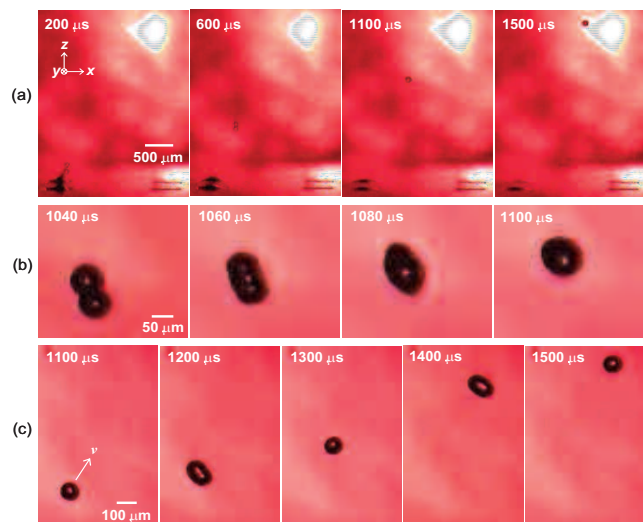
Figure 5. Droplets ejection process (Ejectors 2 and 4 activated). (a) Overview pictures of the ejection process. (b) Detailed droplets coalescence sequence around 1100 \mu s. (c) Rotations of the traveling coalesced droplet with a periodicity of 400 \mu s.
