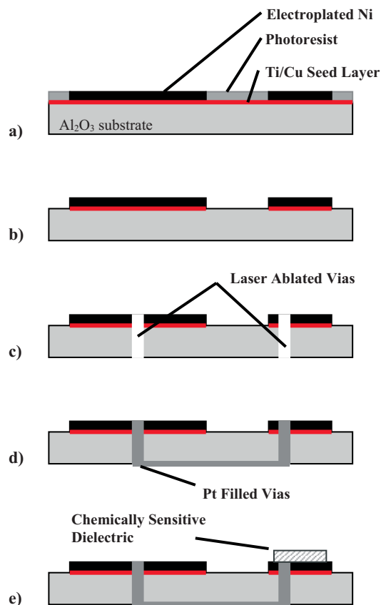
Figure 4. Process flow for sensor fabrication.
