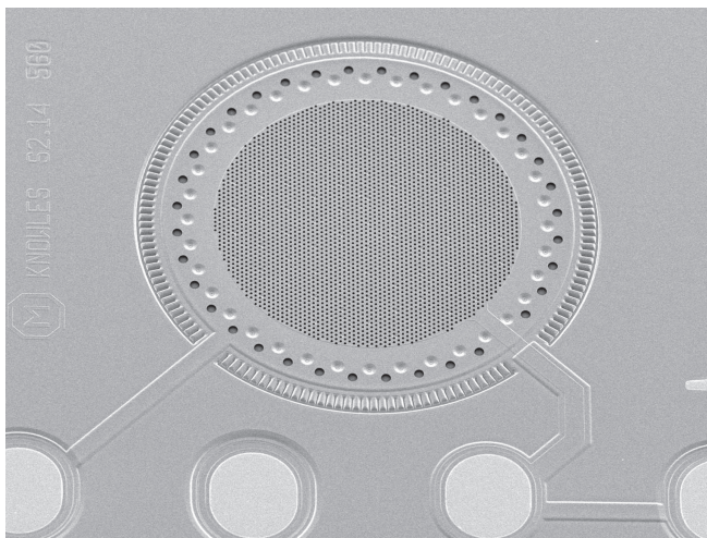
Figure 3. MEMS motor
