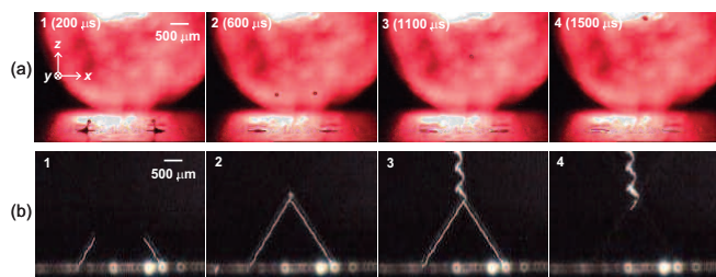
Figure 4. Droplet ejection process captured (a) with and (b) without strobe (Ejectors 1 and 2 activated). Ejectors were driven with \pm 80 - V_{peak-to-peak} pulses of 16- \mu s pulsewidth with 60-Hz pulse repetition frequency (PRF).
