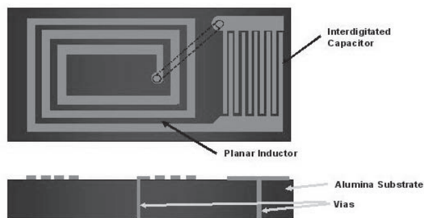
Figure 2. Diagram of wireless sensing platform.
