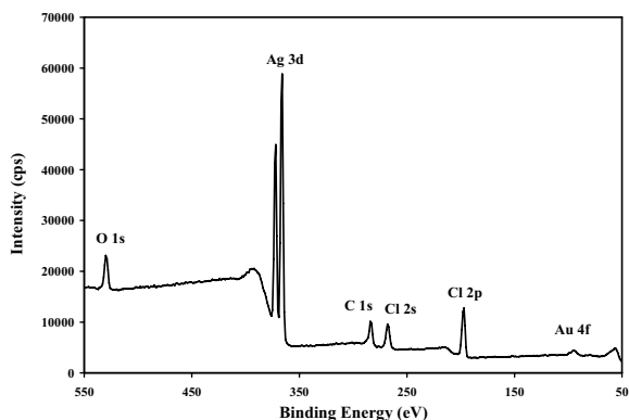
Figure 2: XPS spectra for the electroplated Ag/AgCl layer after treatment in FeCl 3 . The key peaks are shown in the spectra above including the characteristic double peak structure for Ag (3d) indicative of AgCl formation. The Ag/AgCl layer is used as the reference electrode.
