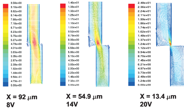
Figure 7. Velocity (m/s) flow patterns within a single slot at a variety of openings ( X ) showing a recirculation zone on the left wall.
