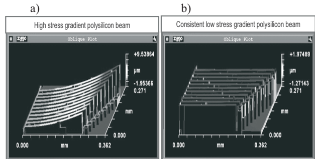
Figure 3. a) Uniform high stress gradient polysilicon with \Delta z > 9\mu m on 350 \mu m poly beam. b) Consistent low stress gradient poly silicon with \Delta z \sim 0.05\mu m on 350 \mu m beam for ULV switch.
