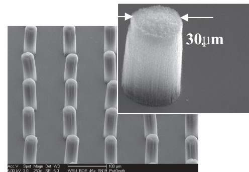
Figure 3. Vertically aligned carbon nanotube arrays.
