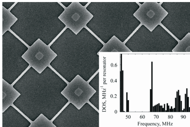
Figure 1. SEM image showing part of the paddle resonator array. The dimensions of the silicon square paddles are 2 \times 2 \mu\text{m} , thickness 45\text{nm} . The SiO 2 pillar supporting the center of the paddle has a cross section 0.54 \times 0.54 \mu\text{m} and is 150\text{nm} tall. The connecting bars are 2 \mu\text{m} long and 200\text{nm} wide. Inset shows the results of finite element analysis for the density of states in the 10 \times 10 paddle array. DOS was calculated by direct counting of the number of modes (deduced from FEM modal analysis) per frequency interval.
