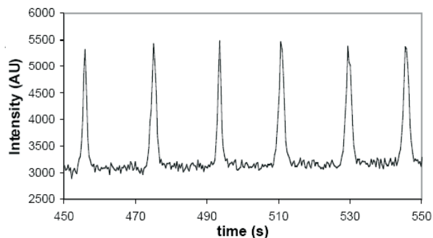
Figure 8 Laser-induced fluorescence (LIF) detection of 1 \mu\text{M} GFP in 10 mM PB injected for 2 s at 600 V from one microfluidic channel, across a NCAM, and into a second microfluidic channel containing the PB solution only.
