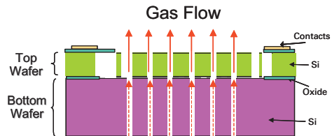
Figure 1. Cross-sectional view of the MEMS gas valve where the middle slider composed of an array of 135 \mu\text{m} wide fingers uncovering the slots of bottom wafer.
