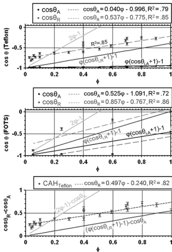
Figure 9: Mode values of advancing and receding contact angles obtained on a) Teflon coated surfaces and b) FOTS coated surfaces are plotted as a function of \phi along with the linear fit lines and model predictions. c) The contact angle hysteresis (CAH) is plotted as a function of \phi for Teflon, as well as model lines and a fit line.
