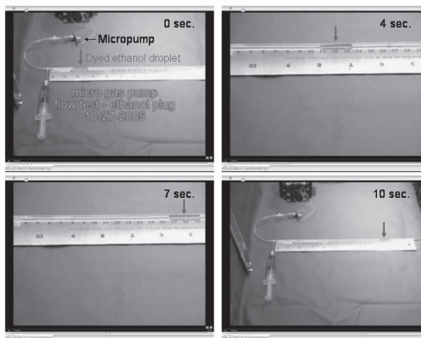
Figure 9: Visualization: ethanol drop is pumped through a thin tube (flow rate: 1.1 sccm) using air being pumped by a gas micro pump.
