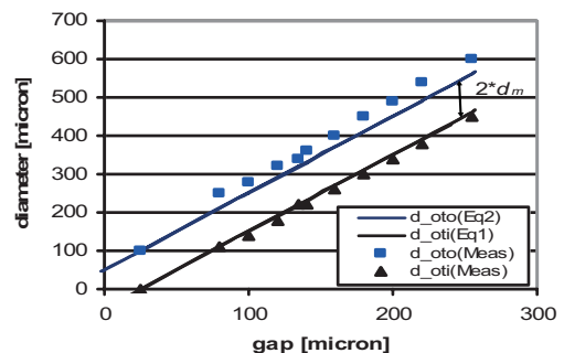
Figure 6. Outer diameter of orifice tip ( d_{oti} ) and inner diameter ( d_{oti} ) as a function of gap
