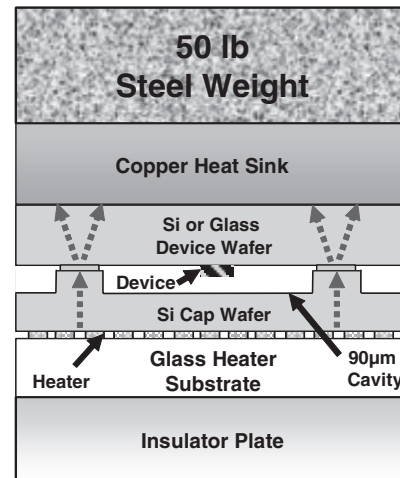
Figure 1: A schematic showing that using the differential heating method, most of the heat flows toward the heat sink as opposed to laterally, towards the device.
