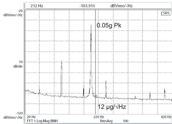
Figure 9. The spectrum of the y-axis output under 0.05g at 200 Hz (RBW = 1Hz).
