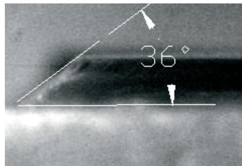
Figure 7. Angle of sidewall of the SU-8 structure
