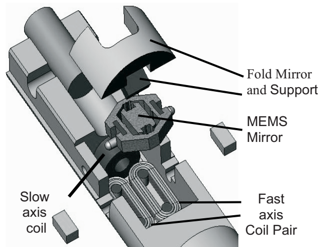
Figure 1. Solid model of endoscope system, showing actuation coils, fold mirror and MEMS mirror.
