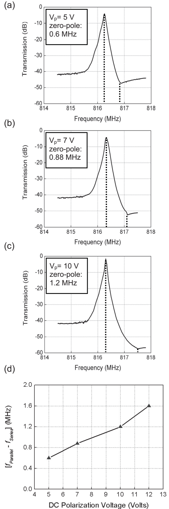
Figure 7. (a, b, c) Measured transmission response demonstrating pole-zero separation of a thickness shear mode resonator as DC bias V_p increases from 5V to 10V. (d) Measured pole-zero separation vs. DC bias voltage of the resonator.
