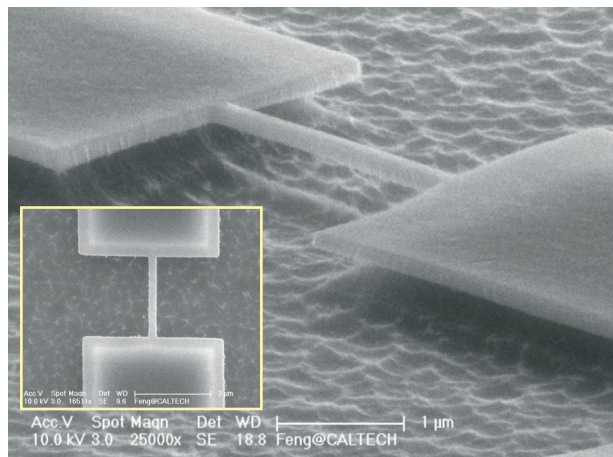
Figure 1. Scanning electron micrographs of a typical single-crystal 3C-SiC UHF NEMS resonator. ( main ) Oblique view (scale bar: 1 \mu\text{m} ) and ( inset ) Top view (scale bar: 2 \mu\text{m} ).
