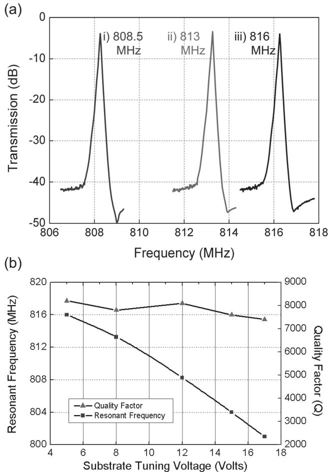
Figure 6. (a) Measured series resonance tuning for V_p = 5 V and V_s = (i) 12 V, (ii) 8 V, and (iii) 5 V. Orthogonal frequency tuning shifts series and parallel resonances by equal amount. (b) Resonant frequency tuning vs. substrate voltage. A tuning range of 15 MHz is observed while maintaining Q > 7000 .
