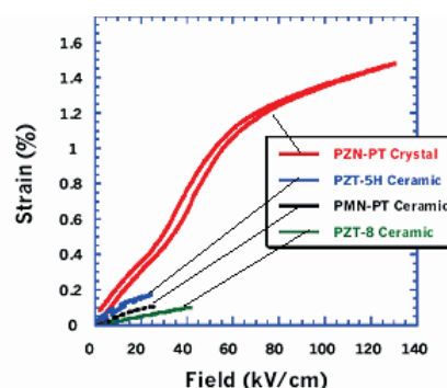
Figure 1. Piezoelectric strain response from single PZN-PT single crystal material compared to piezoelectric and electrostrictive ceramics. The crystal strain remains nearly hysteresis free up to \sim 0.6\% . At high fields very large strains >1\% can be achieved but with an increase in hysteresis.
