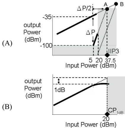
Figure 1. Example of measured range for (A) a two-tone test and (B) a 1 dB compression test. Shaded areas are inaccessible for measurement.
