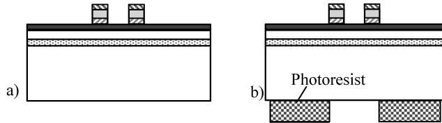
Figure 7: Continuing process steps. a) Wet etch PZT in 3:1:1 of (\text{NH}_4)\text{HF}_2/\text{HCl}/\text{DI} water. b) Spin & pattern thick PR on back.
