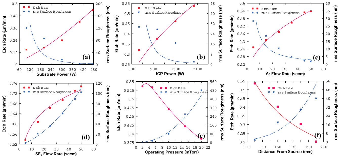
Figure 2: Variation of etch rate and rms surface roughness with (a) Substrate Power, (b) ICP power, (c) Ar flow rate, (d) SF 6 flow rate, (e) operating Pressure and (f) Distance from source for etching of Pyrex. The lines in the graphs are fit to the data and are given by equations 1-6 in the text.
