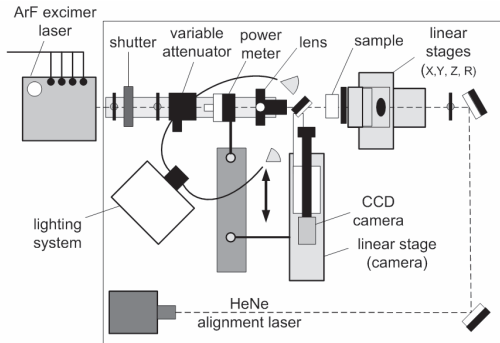
Figure 3. Four-axis laser micromachining system.
