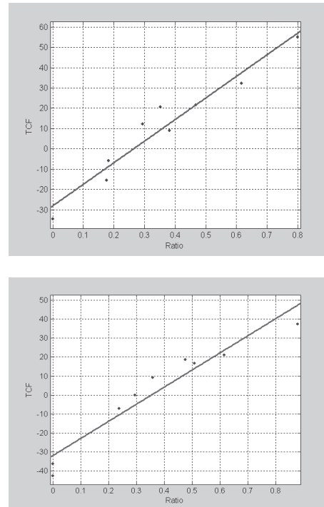
Figure 3 Measured TCF (ppm/°C) at 4.6GHz(top) and 3.4GHz (bottom) vs. the ratio of the +TCF layer thickness to the -TCF layer thickness.
