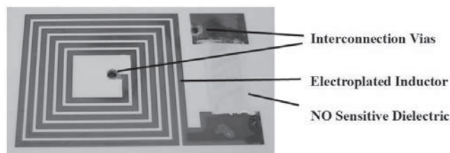
Figure 5. Fabricated sensor with electroplated nickel inductive coil. NO sensitive dielectric stencil printed over capacitor electrodes.
