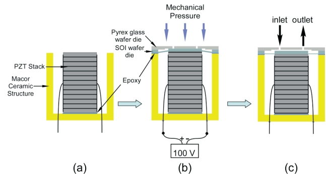
Fig. 5: Prestressed microvalve assembly procedure: (a) First, PZT stack is attached to the Macor ceramic structure using epoxy. (b) Then diced Si-glass die is bonded at the end of PZT and Macor structure by epoxy joint. During this procedure, the PZT stack is actuated until the epoxy is fully cured which results in a normally open valve (c).
