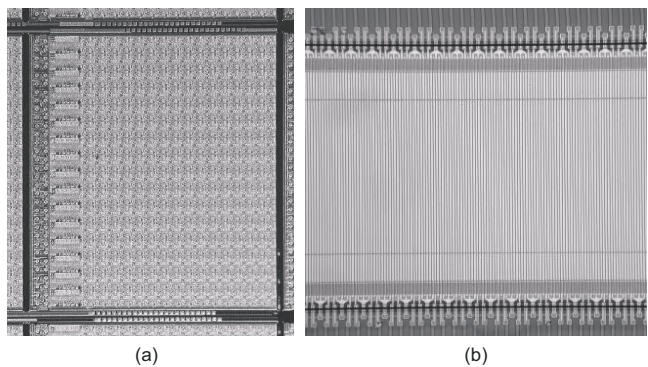
Figure 4. Photograph of the CMOS driver die (a) and a portion of the beam array on the GLV modulator die (b).
