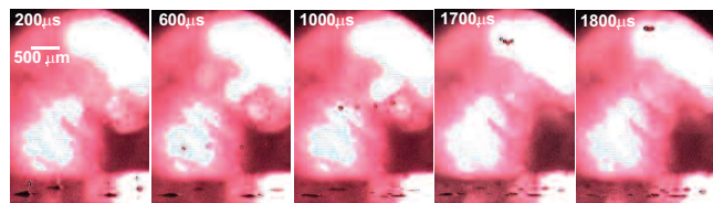
Figure 6. Optical micrographs of the droplets ejection process (all four ejectors activated). Ejectors were driven with \pm 80 - V_{peak-to-peak} pulses of 30- \mu s pulsewidth with 60-Hz PRF.
