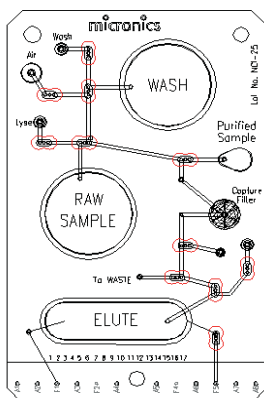
Figure 4. Schematic of nucleic acid extraction subcircuit. The operational steps currently are:
