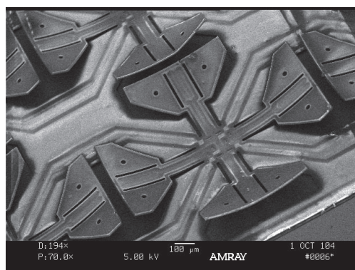
Figure 2. Zoomed-in view of cilia chip fabricated by J. Suh [6] in its unheated state. Resistive heating of a thermo-bimorph cilium decreases its curvature. A “motion pixel” consisting of a group of 4 orthogonal cilia is in the center of the image; independent control of the cilia can generate force or motion in 4 orthogonal directions.
