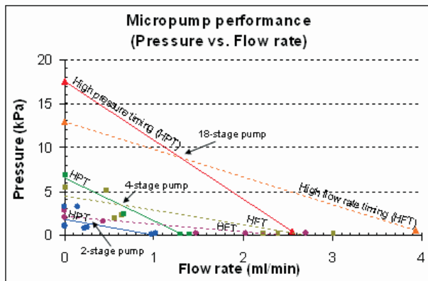
Figure 8: Pressure versus flow rate measurement results of different number of stage micropumps.
