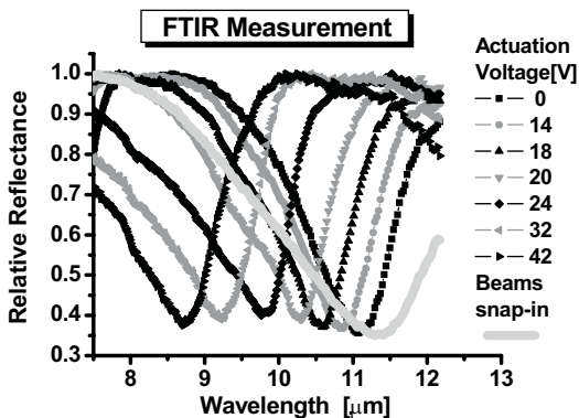
Figure 5. FTIR measurement of the relative reflectance spectra of a 120 by 120 \mu\text{m} square filter. As the applied voltage is varied from 0 – 42 \text{V} , the narrowband resonance shifts from 11.1 \mu\text{m} to 8.7 \mu\text{m} . A broadband resonance centered at 11.3 \mu\text{m} is created when the voltage is increased to 45 \text{V} .
