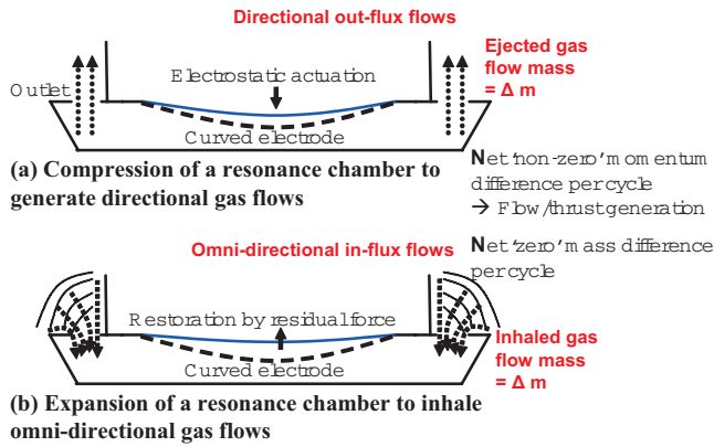
Figure 2. Operation principle of the electrostatic acoustic microjet generator.
