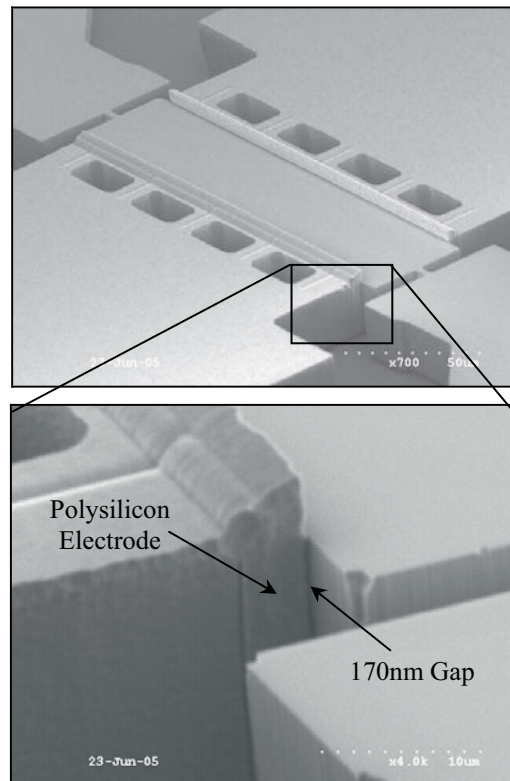
Figure 1. SEM view of a 40\mu\text{m} wide, 150\mu\text{m} long, 20\mu\text{m} thick clamped-clamped SiBAR and the close up of its electrode showing the 170\text{nm} capacitive gap.
