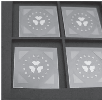
Figure 5. Photographs of the MEMS mirror (left) and baseplate (right) for a digital MEMS optical switch.
