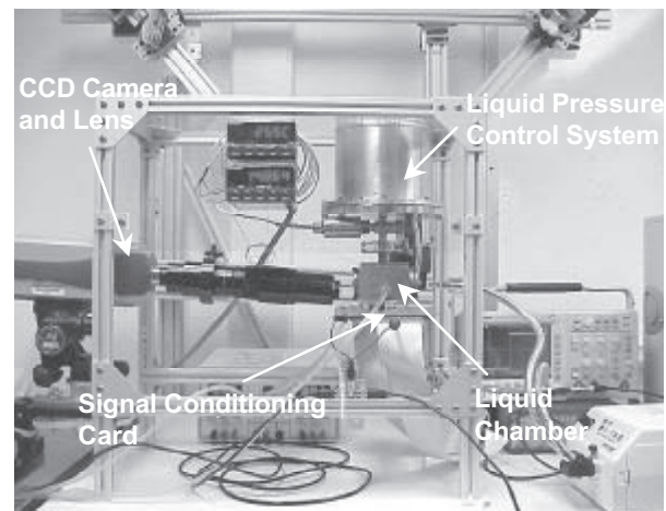
Figure 5. Experimental setup
