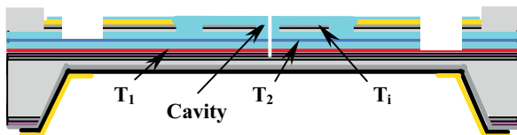
Figure 1. Cross section of the device.
