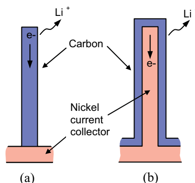
Fig. 2 Schematic of deintercalation of Li-ion in carbon post anode during discharge. (a): Previously reported carbon post suffers from the high potential drop along the slender carbon post at high discharge rates. (b): Our design of carbon post has minimized potential drop through its metal core, while maintaining the carbon as the anodic material
