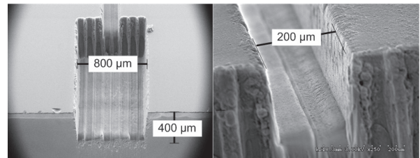
Figure 7. Laser milling on Pyrex realized with optimal parameters and circular beam overlap strategy ( F=6 \text{ J}/\text{cm}^2, f=100 \text{ Hz}, V=170 \mu\text{m/s}, N=40 \times 8 for rectangular cavity, machining time: 3 hours).
