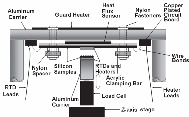
Figure 4. Schematic of steady state heat transfer experiments.
