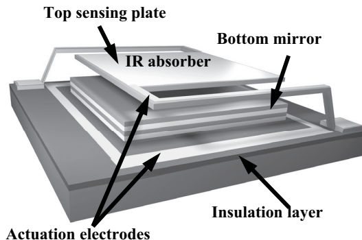
Figure 1. Conceptual diagram of a tunable absorption filter for LWIR microbolometers. The primary actuation electrodes are on the support beams and substrate to delay snap-through and enhance tuning range.
