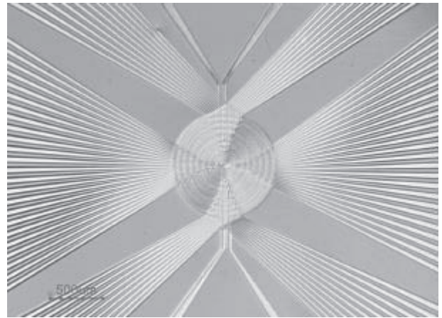
Figure 3. Wide view of the device showing leads of the sensor array and two pairs of leads for sensors T_1 and T_2 .
