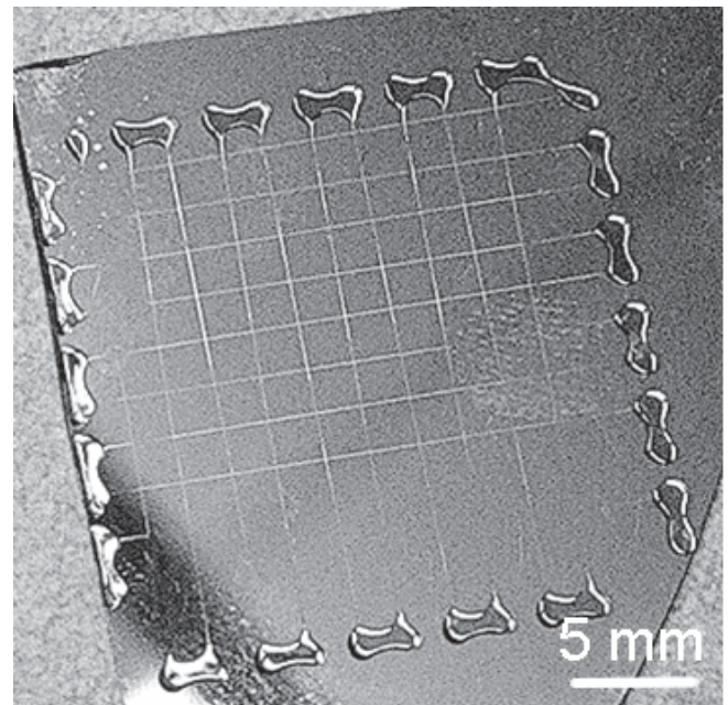
Figure 6. Pattern generated with direct-write method.
