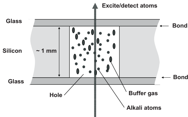
Figure 2. Design of a MEMS-based alkali atom vapor cell for chip-scale atomic devices.
