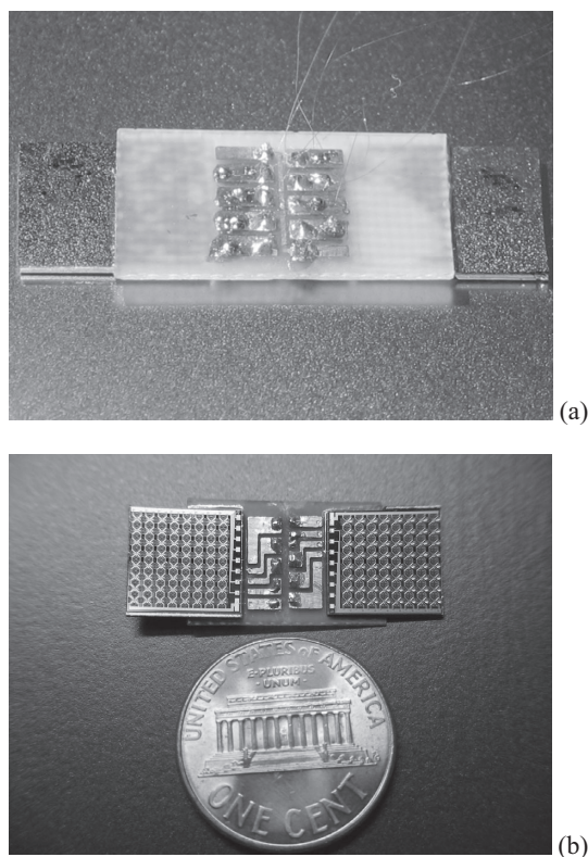
Figure 1. (a) Top and (b) bottom view of the microrobot. The two cilia chips can be seen attached and wire bonded to a PCB backbone. Each chip consists of an 8 \times 8 array of “motion pixels” (i.e., a group of 4 orthogonal cilia). The robot measures approximately 3cm length, 1cm width and 0.5mm thickness.
