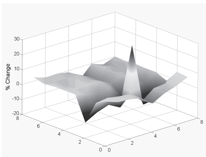
Figure 6: Graph of change in capacitance of array when loaded by a 3mm spherical indenter. X and Y axes are the row and columns of the capacitive array.
